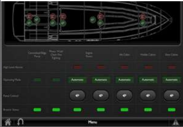
Representation of a bilge system.
